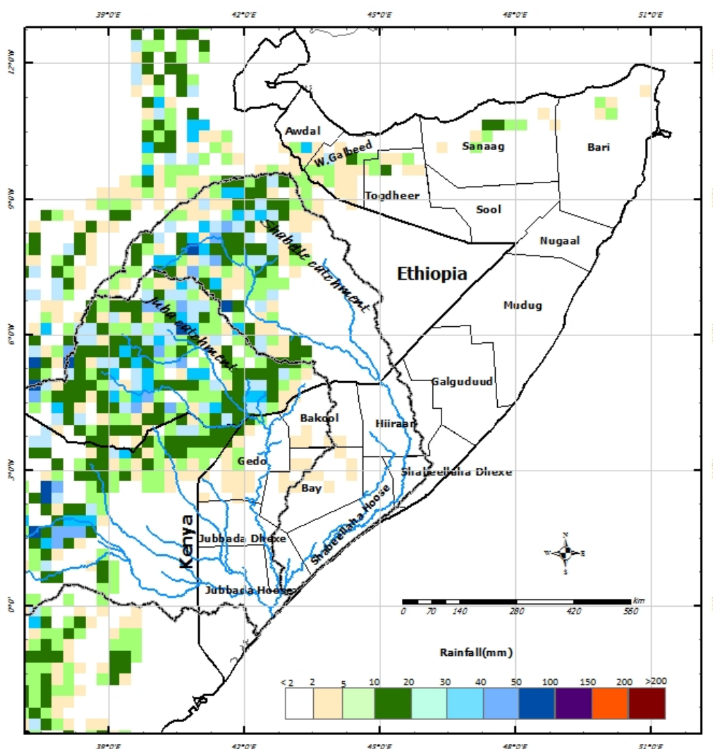
24 hours total rainfall forecast valid on 06/04/2016
