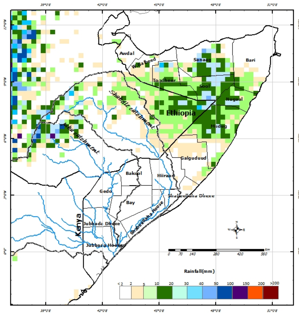
3-day accumulated rainfall forecast (12/10/2016 to 14/10/2016)
