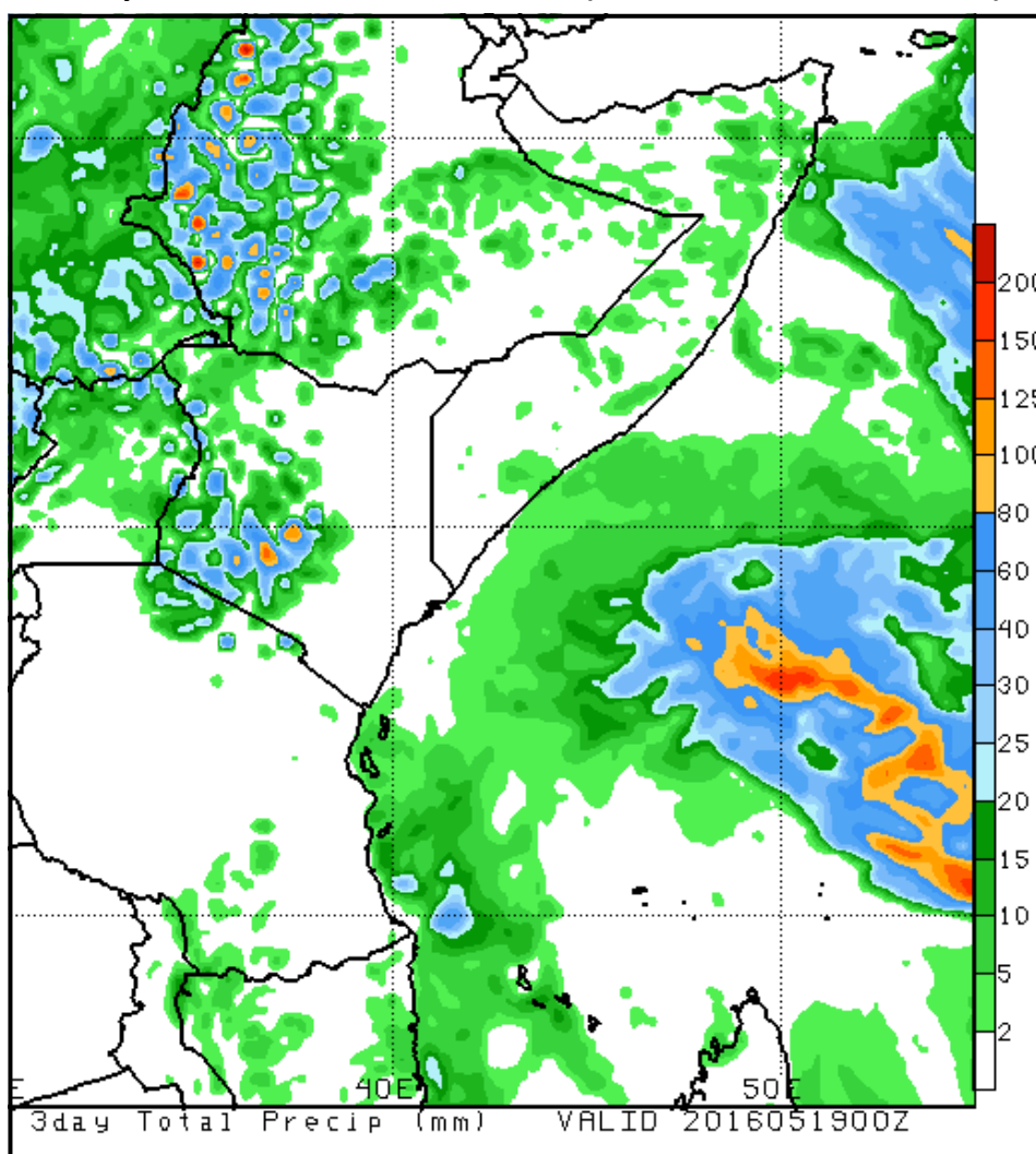
3-day accumulated rainfall forecast (17/05/2016 to 19/05/2016)
