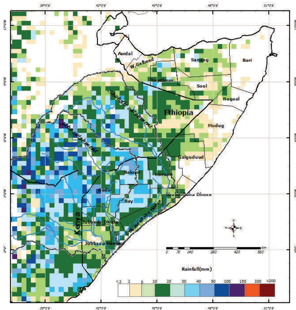
3-day accumulated rainfall forecast (30/10/2015 to 01/11/2015)
